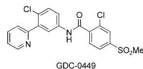
Scheme 12. Structure of GDC-0449.
