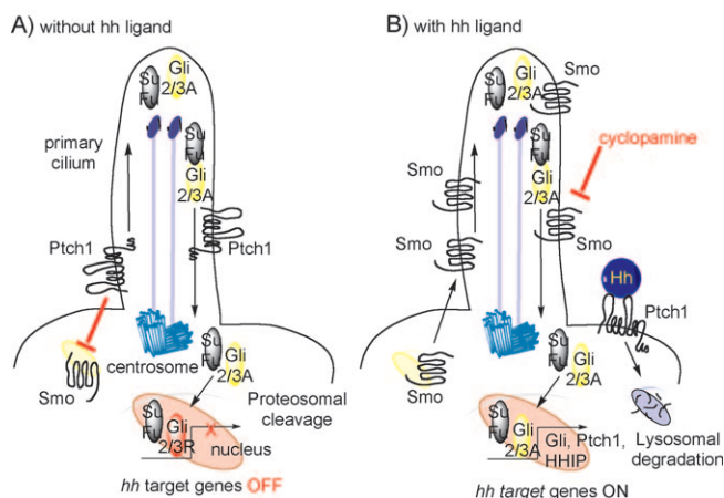
Figure 1. The hedgehog signaling pathway. A) In the absence of hh ligands, Ptch1 inhibits Smo from entering the cilium; thus, SuFu stays active, the Gli2/3 transcription factors are cleaved by proteasomes, and transcription of hh -target genes is prevented. B) The binding of a hh ligand results in Ptch1 being inhibited and Smo moves into the cilium, where SuFu is inhibited and the active form of the Gli2/3 factors can activate transcription of the hh gene in the nucleus; cyclopamine inhibits the activity of Smo and leads to deactivation of the hh path. For further explanation, see the text; scheme modified from Ref. [14b].
